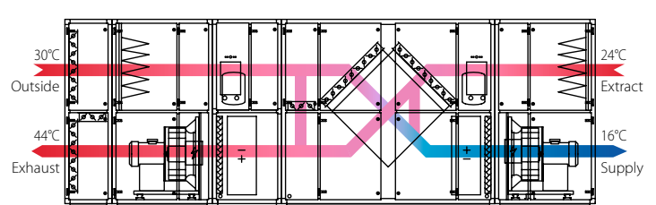
Heat exchanger pre-cooling outside air. Compressor activity 100% (system running in cooling mode). PRS supply air temperature control activated.
